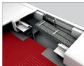
cross section - guide track with zip system and internal PVC profile with vario belt
