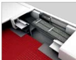
cross section - guide track with zip system and internal PVC profile with vario belt
